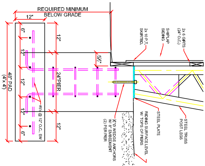
SECTION @ STEEL POST PIERS SCALE: 1" = 1'-0"
